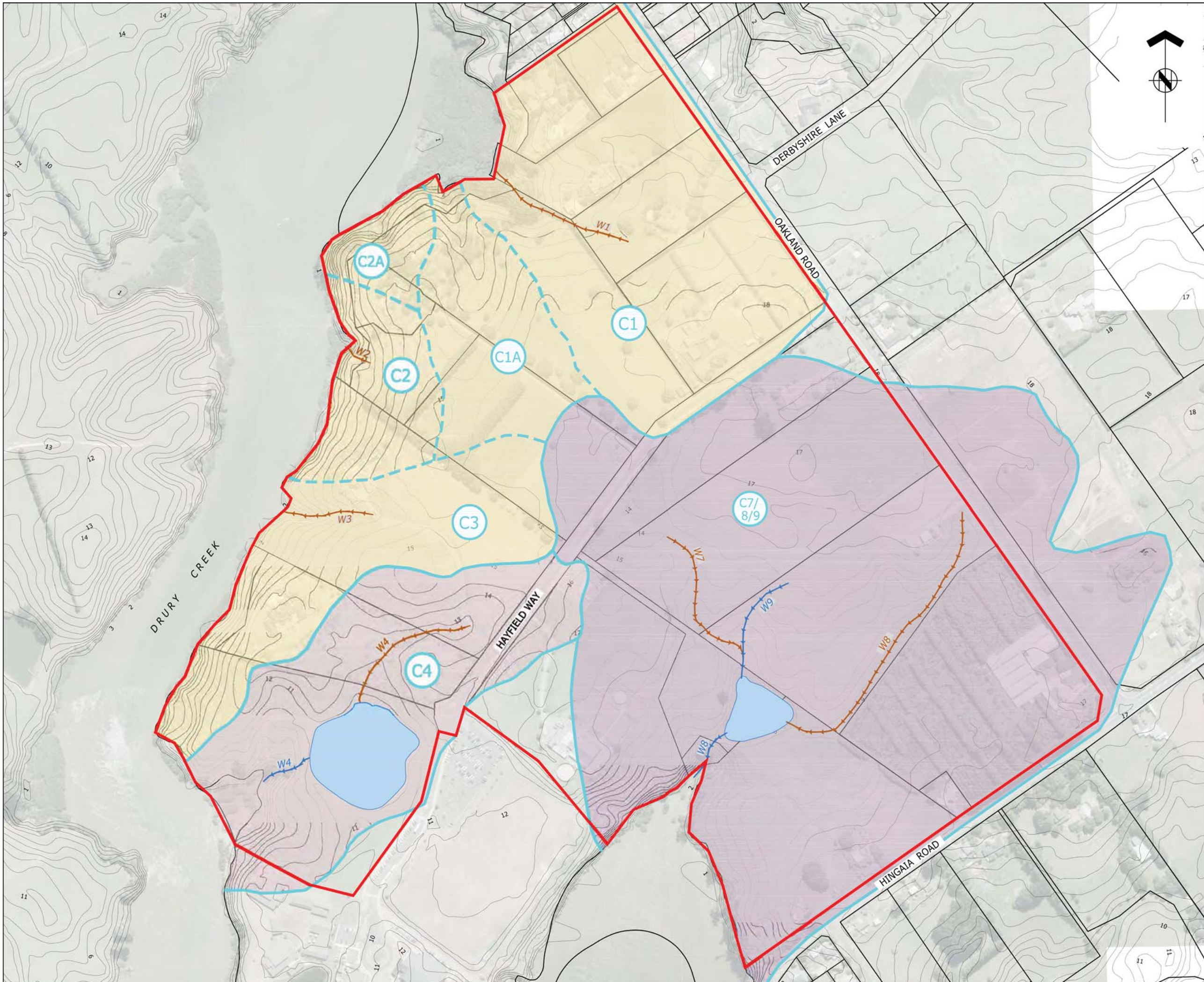
Figure 3a - Existing Stormwater Catchments Plan
